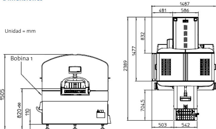
AUTOMAC 40 ZS - In line
